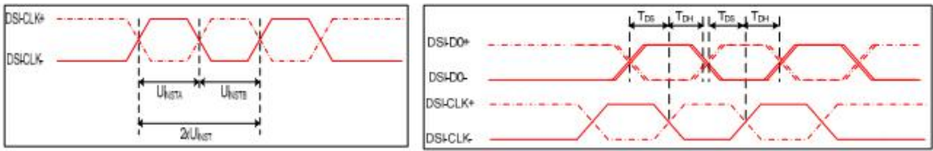
Figure 5.3.1 clock channel timing
