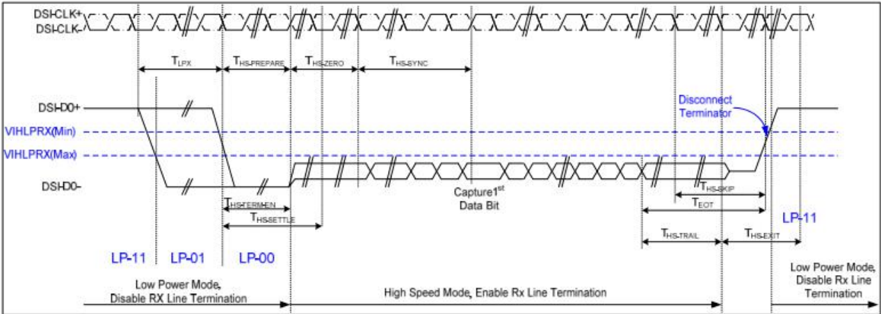
Figure 5.3.3 High speed data transmission timing sequence
