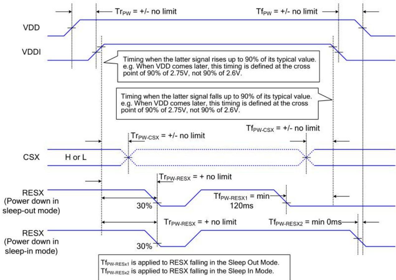
Figure 5.5.1 VCI/VDDI input power on/of sequence
